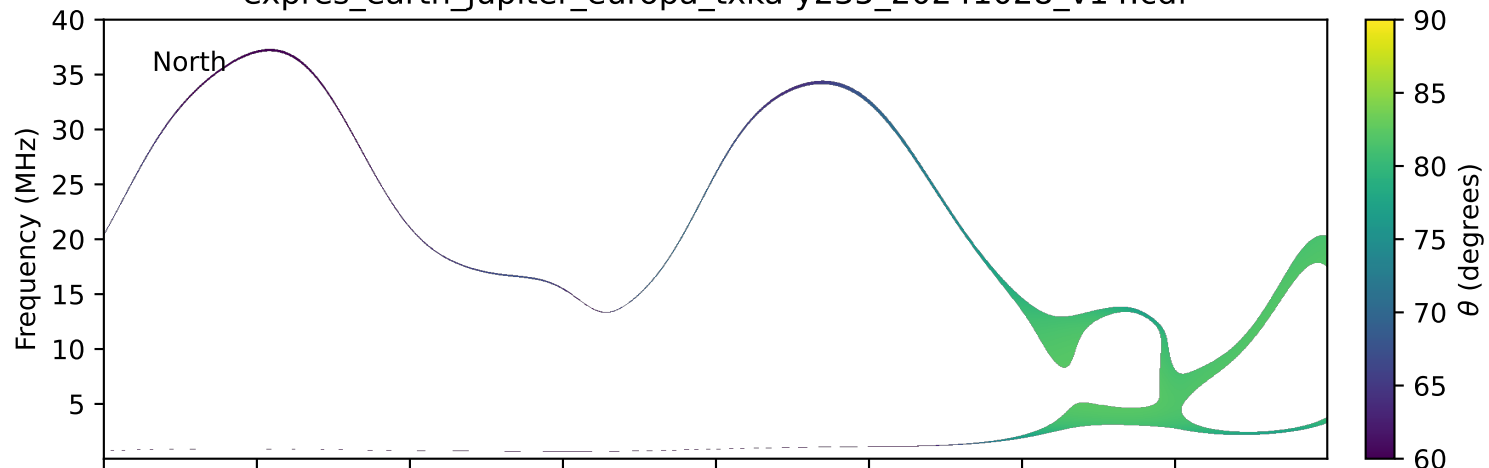
expres_earth_jupiter_europa_txka-y235_20241028_v14.cdf
