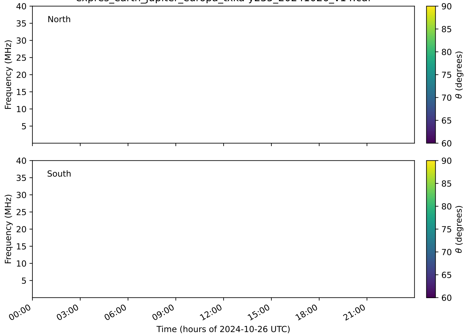
expres_earth_jupiter_europa_txka-y235_20241026_v14.cdf
