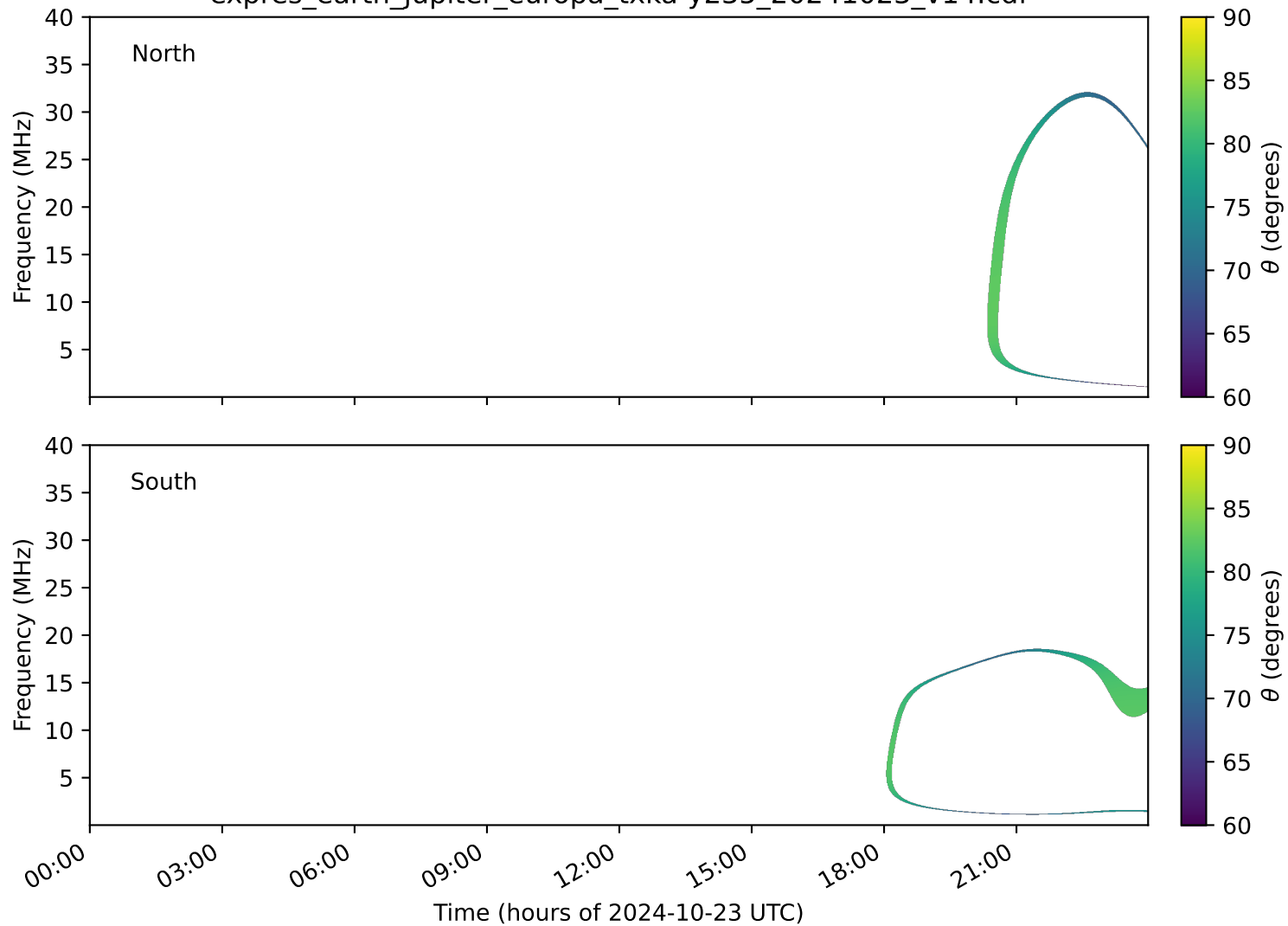
expres_earth_jupiter_europa_txka-y235_20241023_v14.cdf
