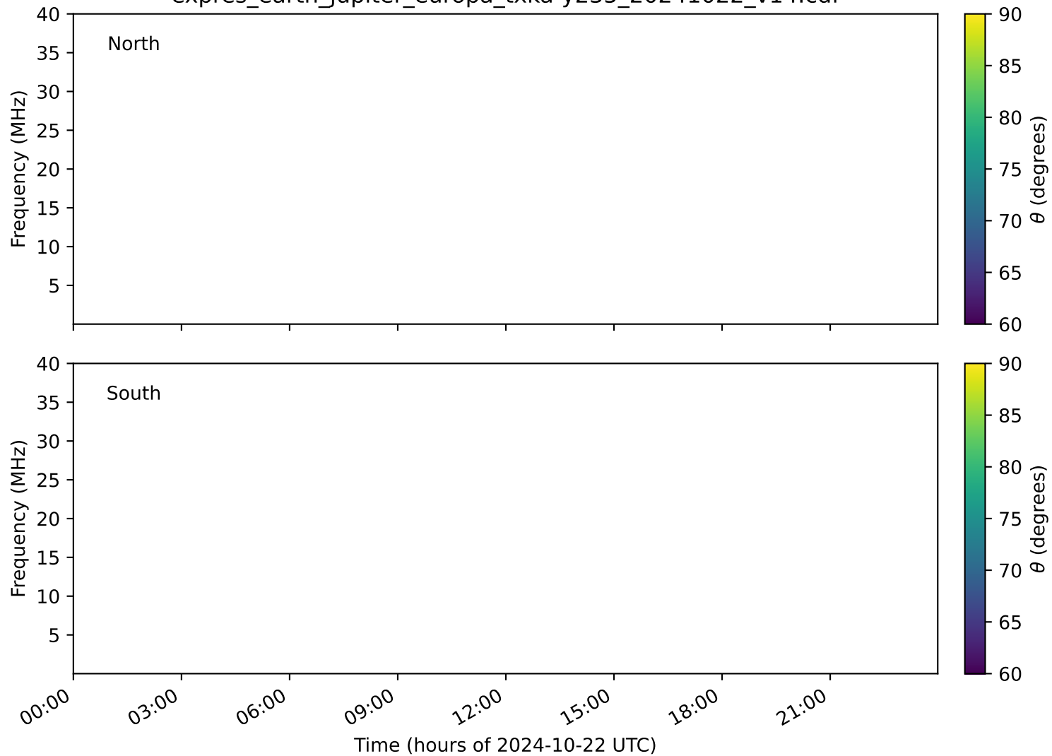
expres_earth_jupiter_europa_txka-y235_20241022_v14.cdf
