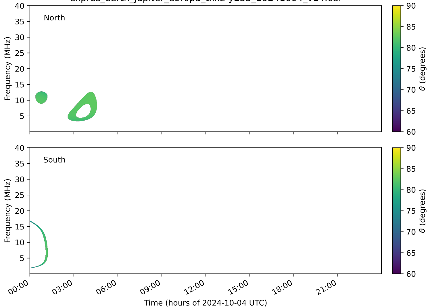
expres_earth_jupiter_europa_txka-y235_20241004_v14.cdf
