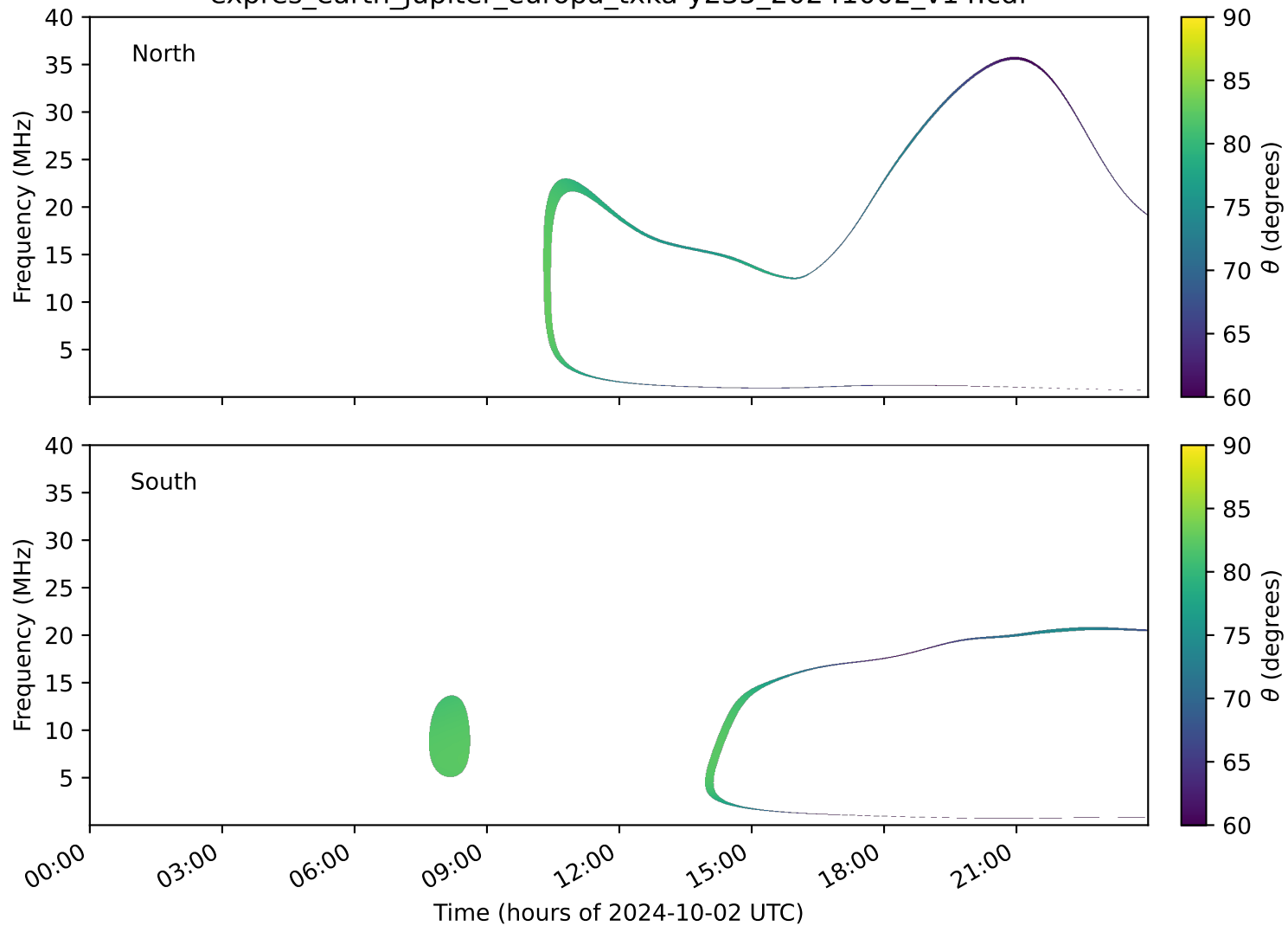
expres_earth_jupiter_europa_txka-y235_20241002_v14.cdf
