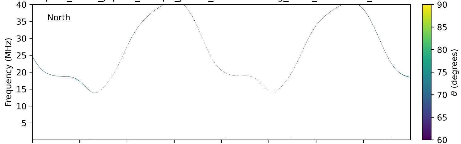
expres_earth_jupiter_europa_jrm33_lossc-wid1deg_3kev_20241017_v11.cdf
