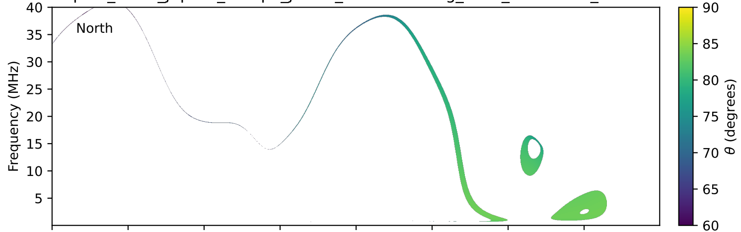
expres_earth_jupiter_europa_jrm33_lossc-wid1deg_3kev_20241014_v11.cdf
