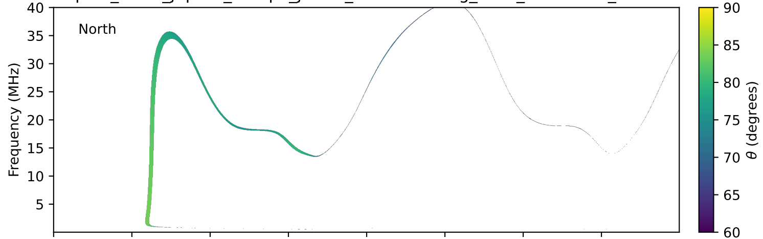
expres_earth_jupiter_europa_jrm33_lossc-wid1deg_3kev_20241013_v11.cdf
