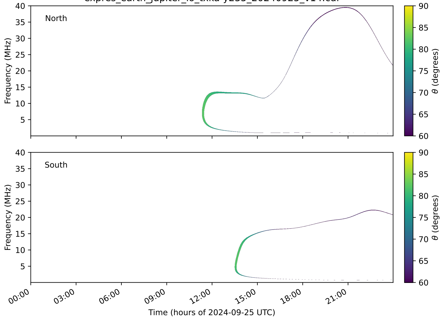
expres_earth_jupiter_io_txka-y235_20240925_v14.cdf
