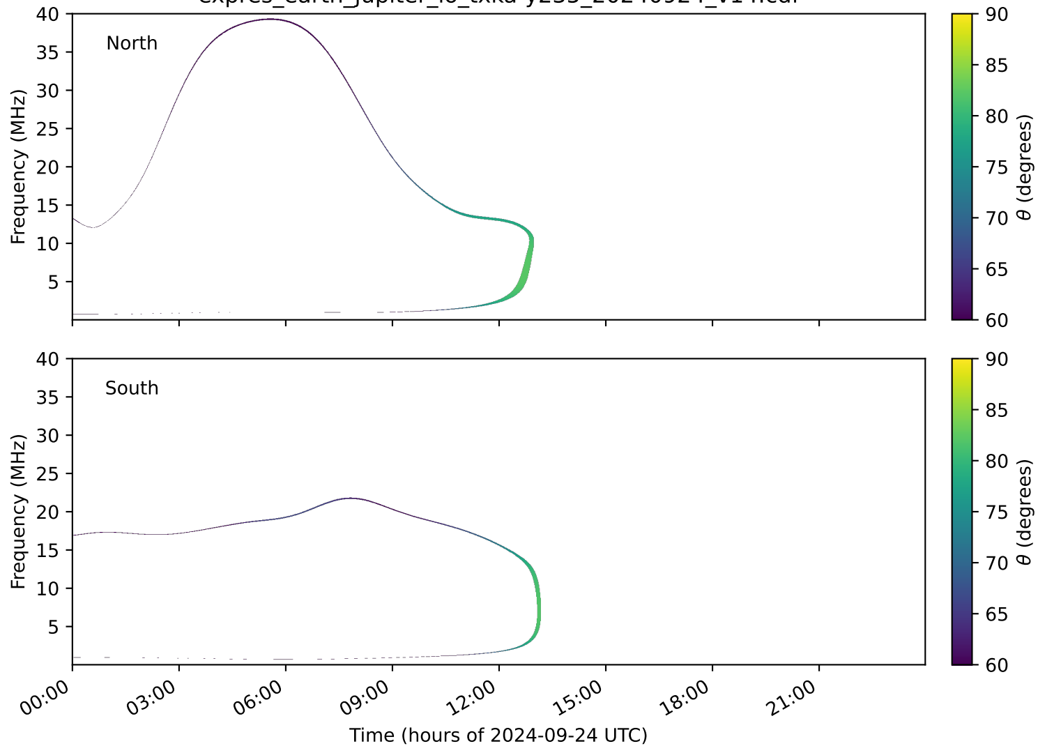
expres_earth_jupiter_io_txka-y235_20240924_v14.cdf
