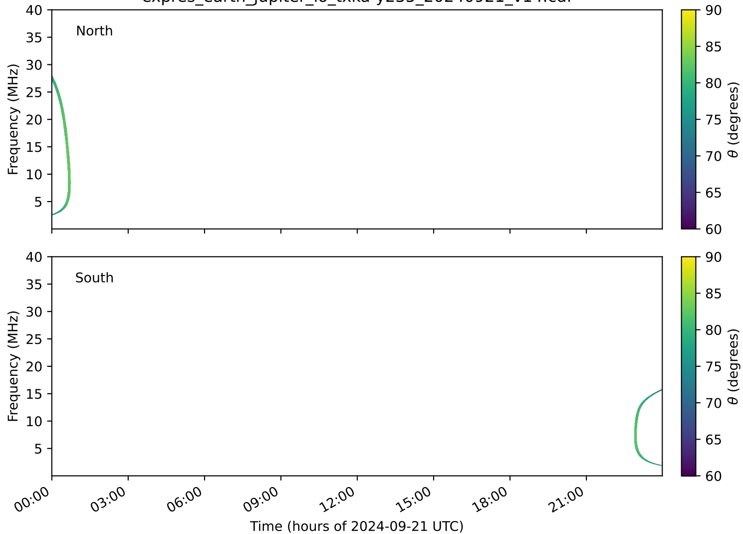
expres_earth_jupiter_io_txka-y235_20240921_v14.cdf
