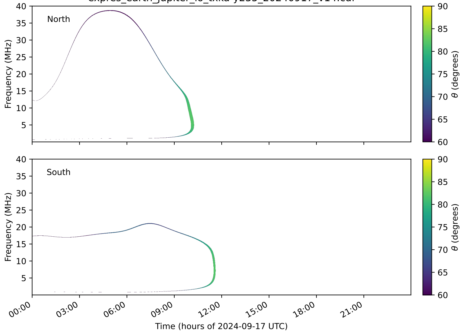
expres_earth_jupiter_io_txka-y235_20240917_v14.cdf
