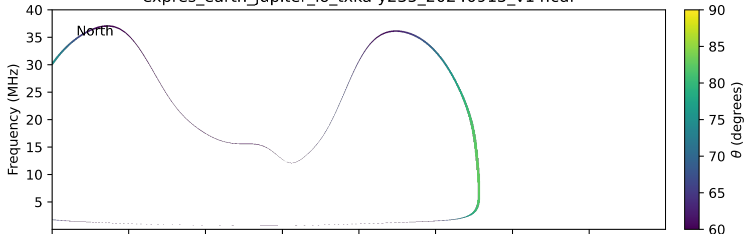
expres_earth_jupiter_io_txka-y235_20240915_v14.cdf
