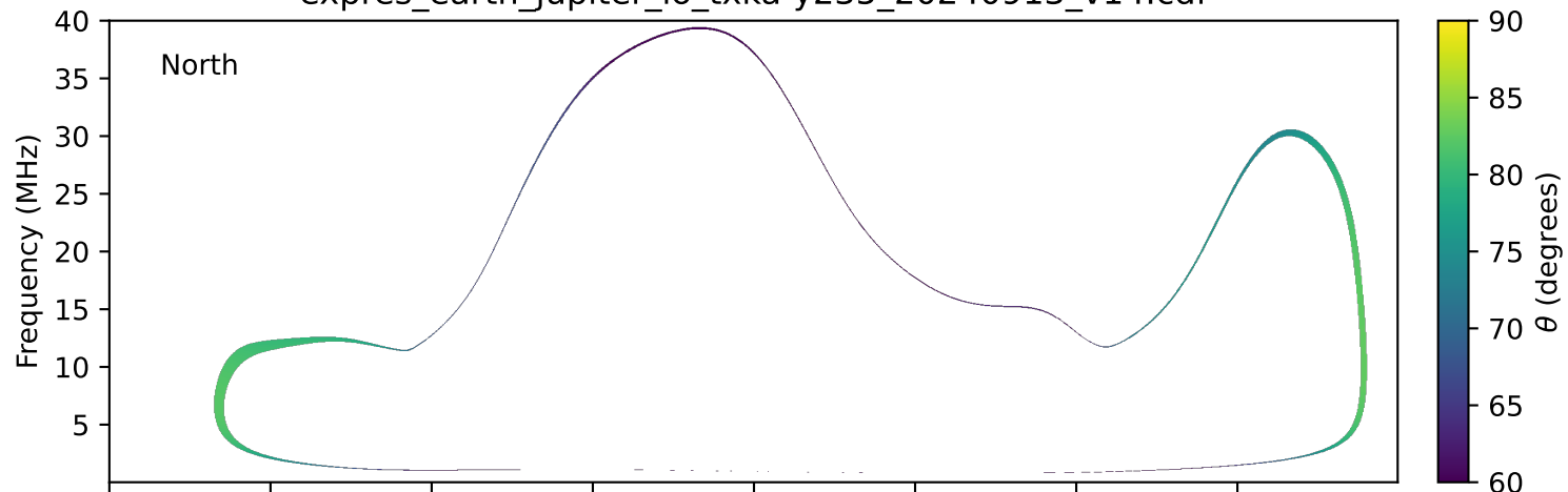
expres_earth_jupiter_io_txka-y235_20240913_v14.cdf
