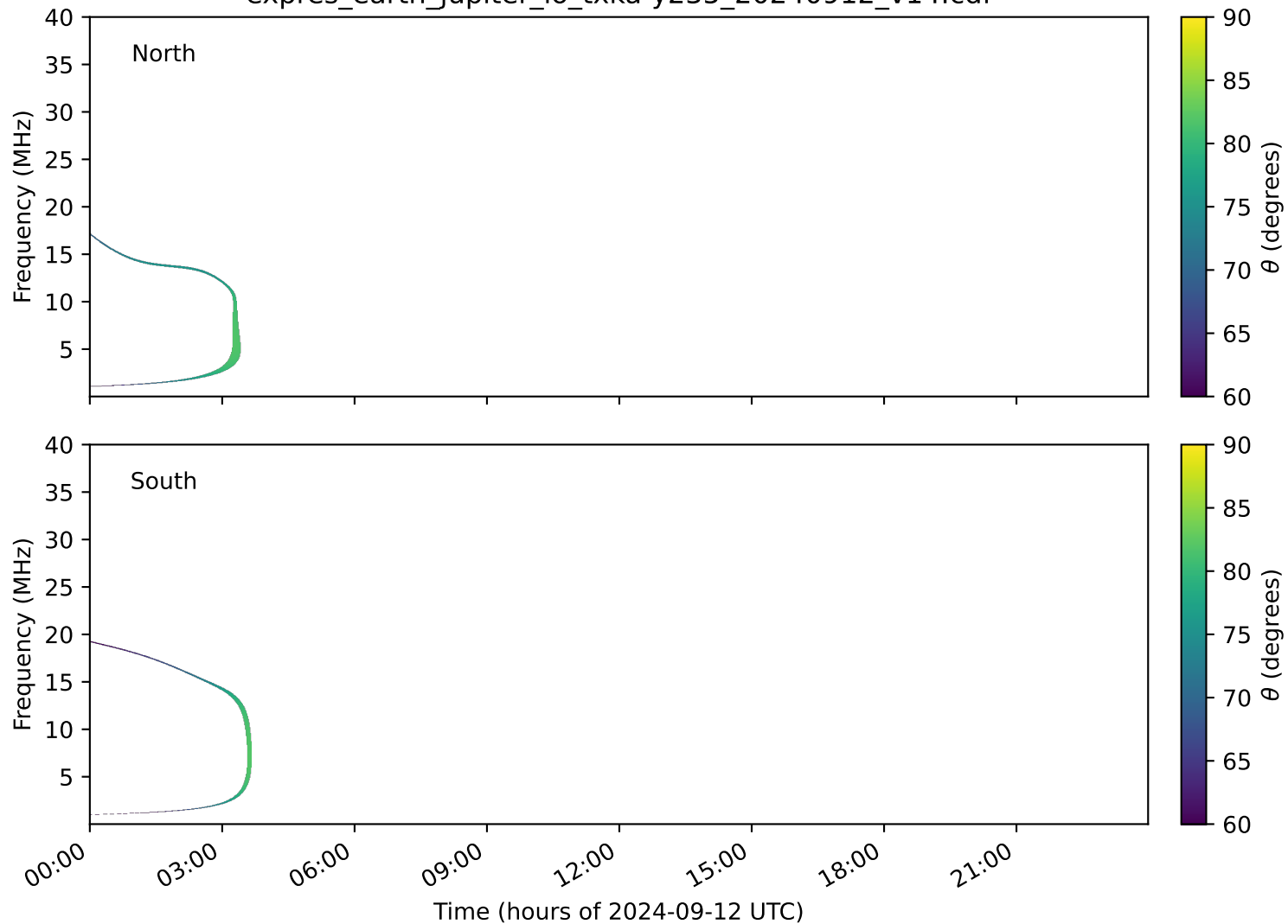
expres_earth_jupiter_io_txka-y235_20240912_v14.cdf
