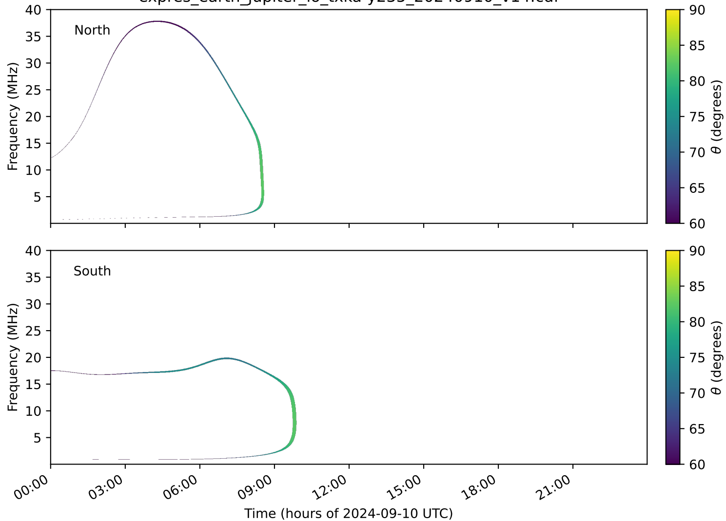
expres_earth_jupiter_io_txka-y235_20240910_v14.cdf
