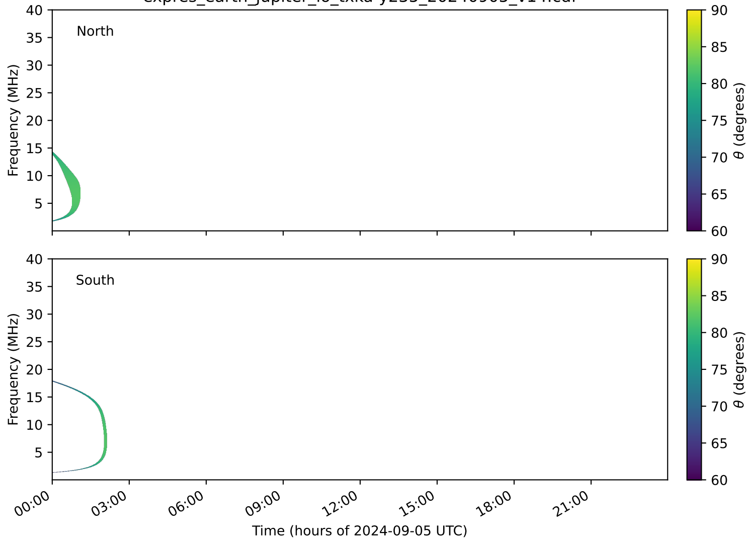
expres_earth_jupiter_io_txka-y235_20240905_v14.cdf
