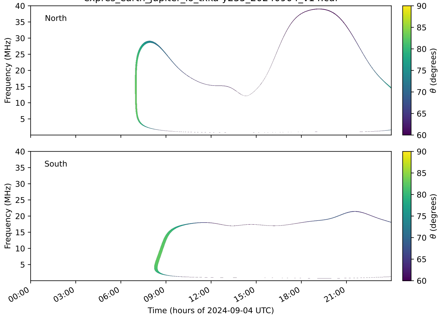
expres_earth_jupiter_io_txka-y235_20240904_v14.cdf
