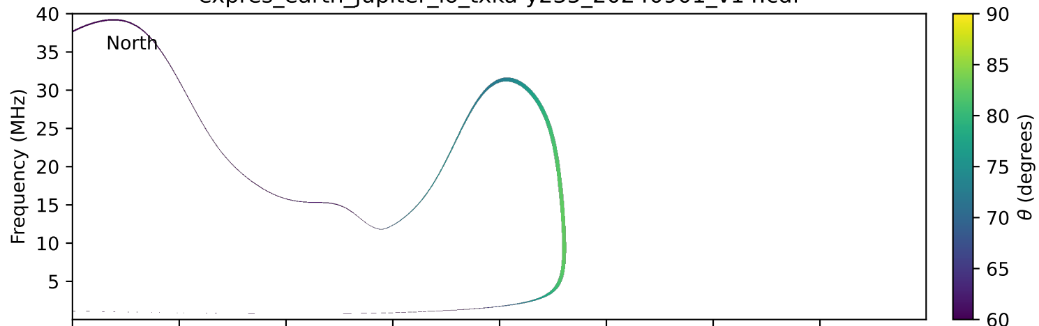
expres_earth_jupiter_io_txka-y235_20240901_v14.cdf
