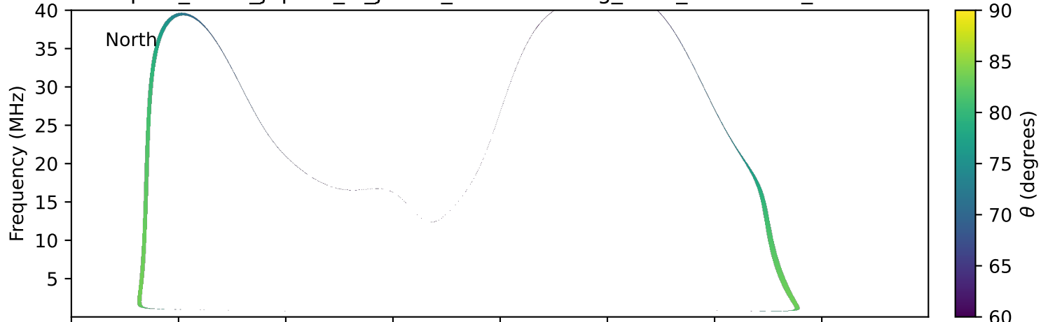
expres_earth_jupiter_io_jrm33_lossc-wid1deg_3kev_20240929_v11.cdf
