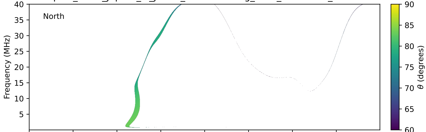
expres_earth_jupiter_io_jrm33_lossc-wid1deg_3kev_20240927_v11.cdf
