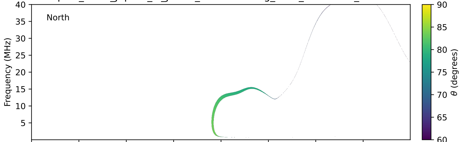
expres_earth_jupiter_io_jrm33_lossc-wid1deg_3kev_20240925_v11.cdf
