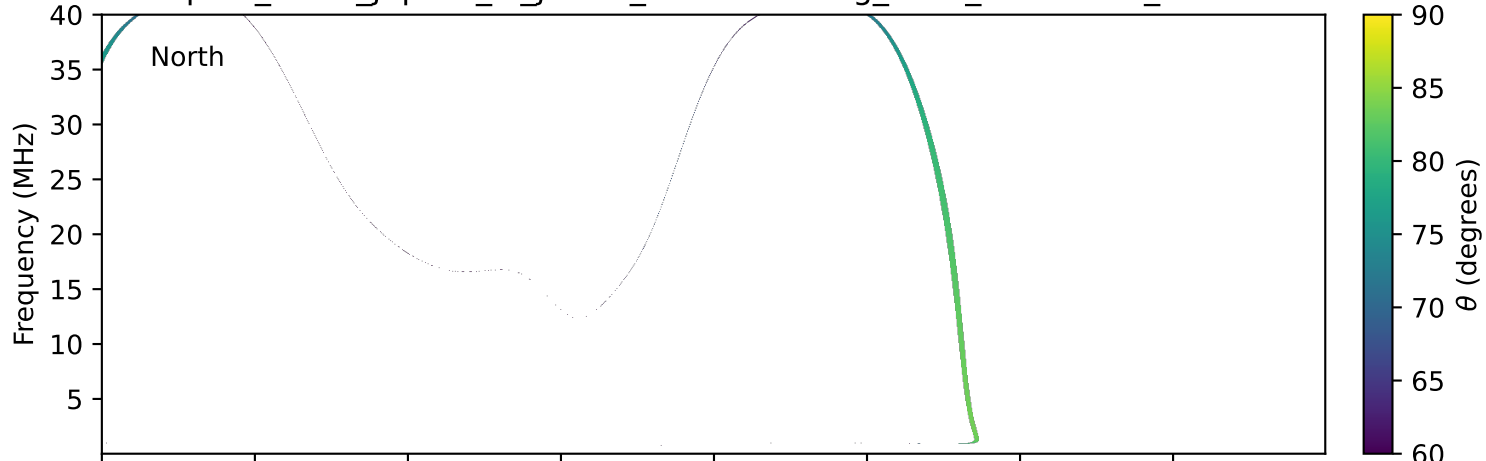
expres_earth_jupiter_io_jrm33_lossc-wid1deg_3kev_20240915_v11.cdf
