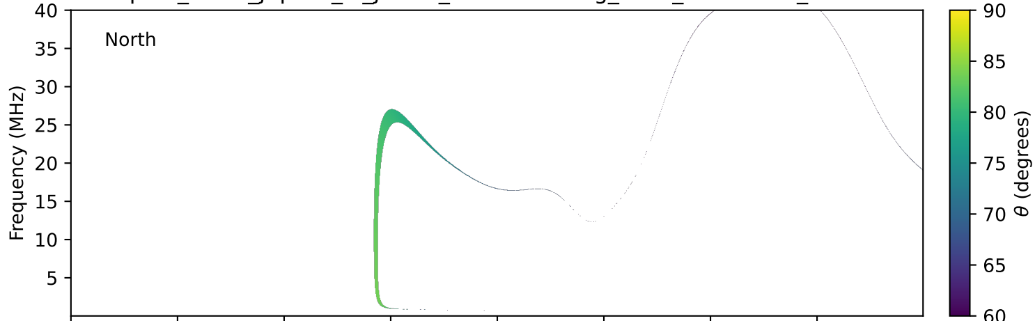
expres_earth_jupiter_io_jrm33_lossc-wid1deg_3kev_20240911_v11.cdf
