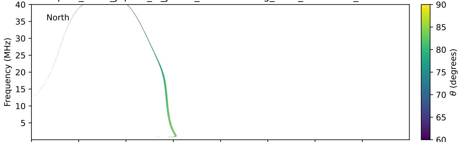
expres_earth_jupiter_io_jrm33_lossc-wid1deg_3kev_20240910_v11.cdf
