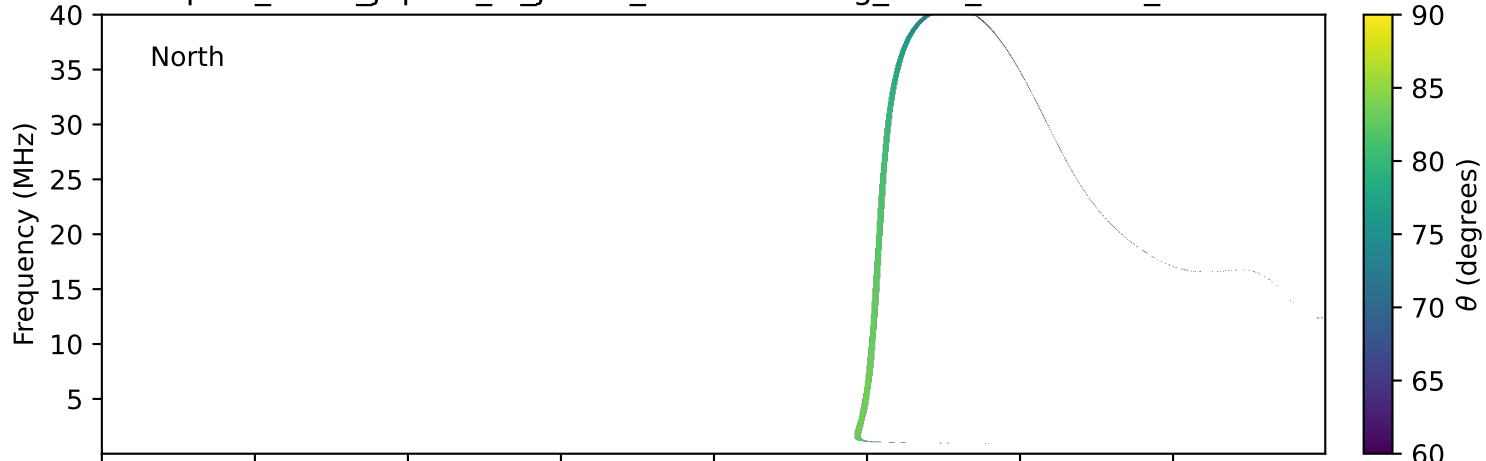
expres_earth_jupiter_io_jrm33_lossc-wid1deg_3kev_20240909_v11.cdf
