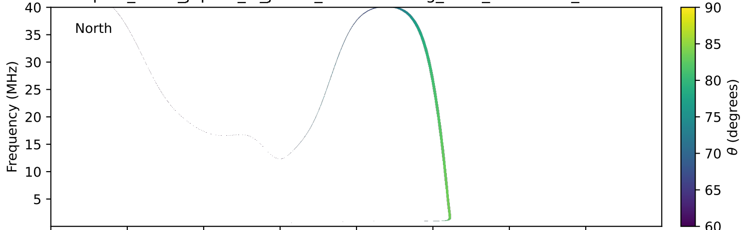
expres_earth_jupiter_io_jrm33_lossc-wid1deg_3kev_20240908_v11.cdf
