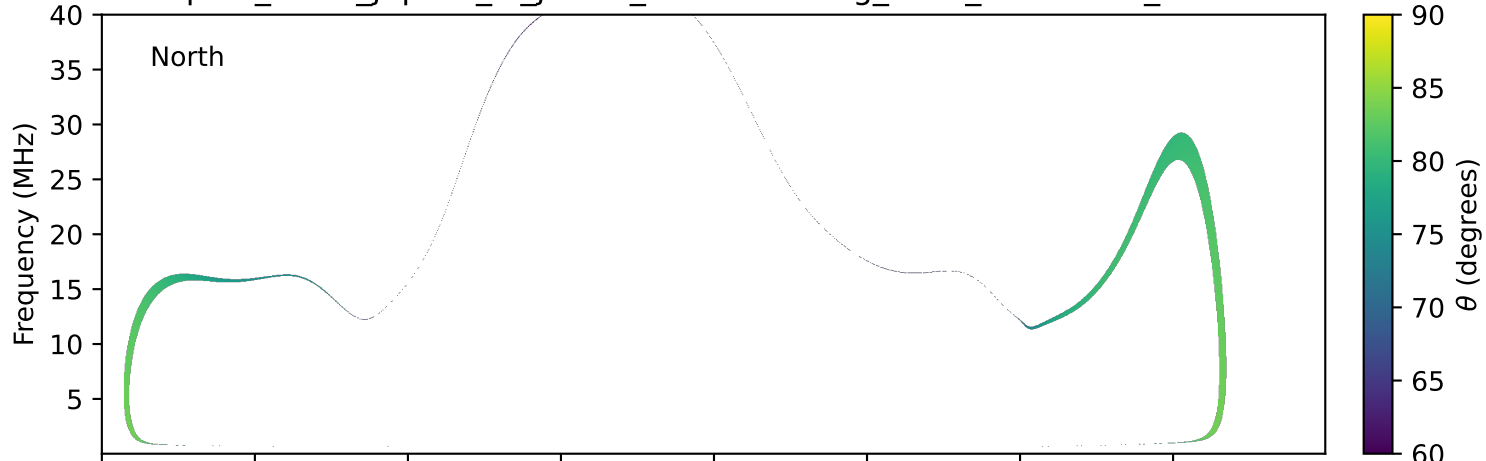
expres_earth_jupiter_io_jrm33_lossc-wid1deg_3kev_20240906_v11.cdf
