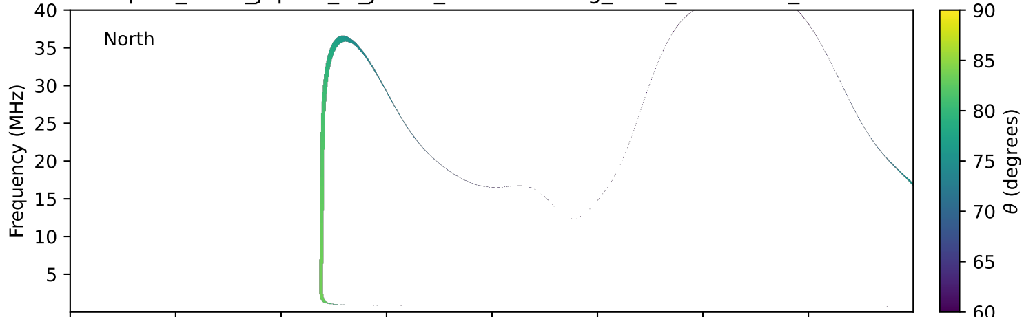
expres_earth_jupiter_io_jrm33_lossc-wid1deg_3kev_20240904_v11.cdf
