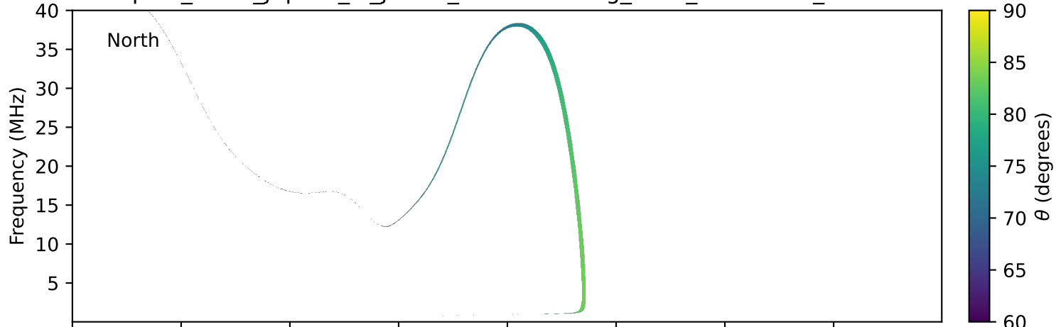
expres_earth_jupiter_io_jrm33_lossc-wid1deg_3kev_20240901_v11.cdf
