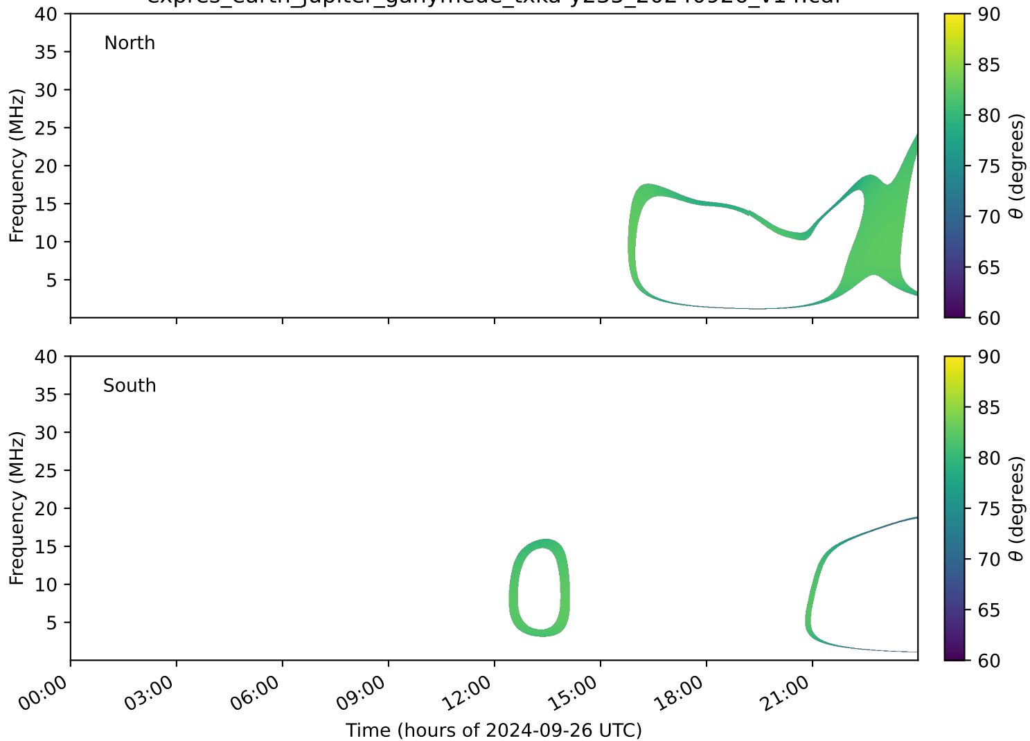
expres_earth_jupiter_ganymede_txka-y235_20240926_v14.cdf
