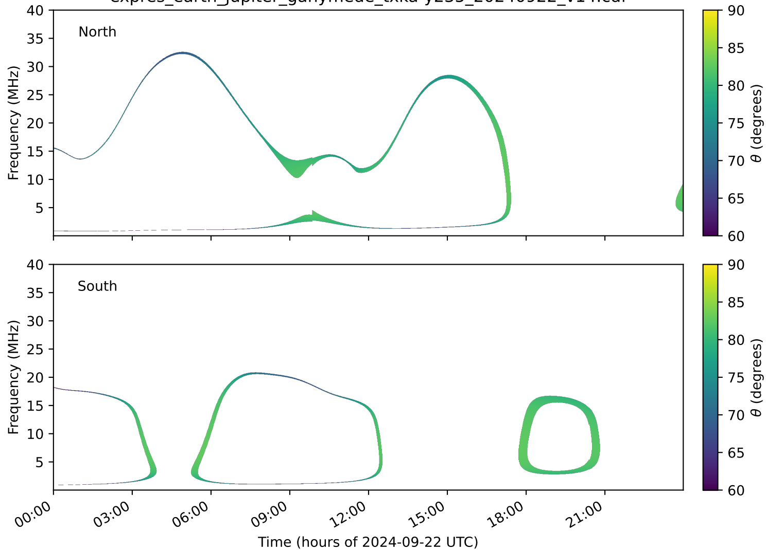
expres_earth_jupiter_ganymede_txka-y235_20240922_v14.cdf
