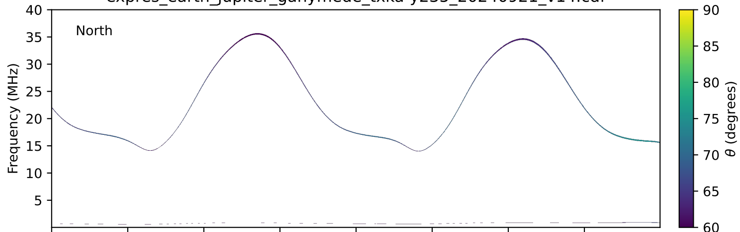
expres_earth_jupiter_ganymede_txka-y235_20240921_v14.cdf
