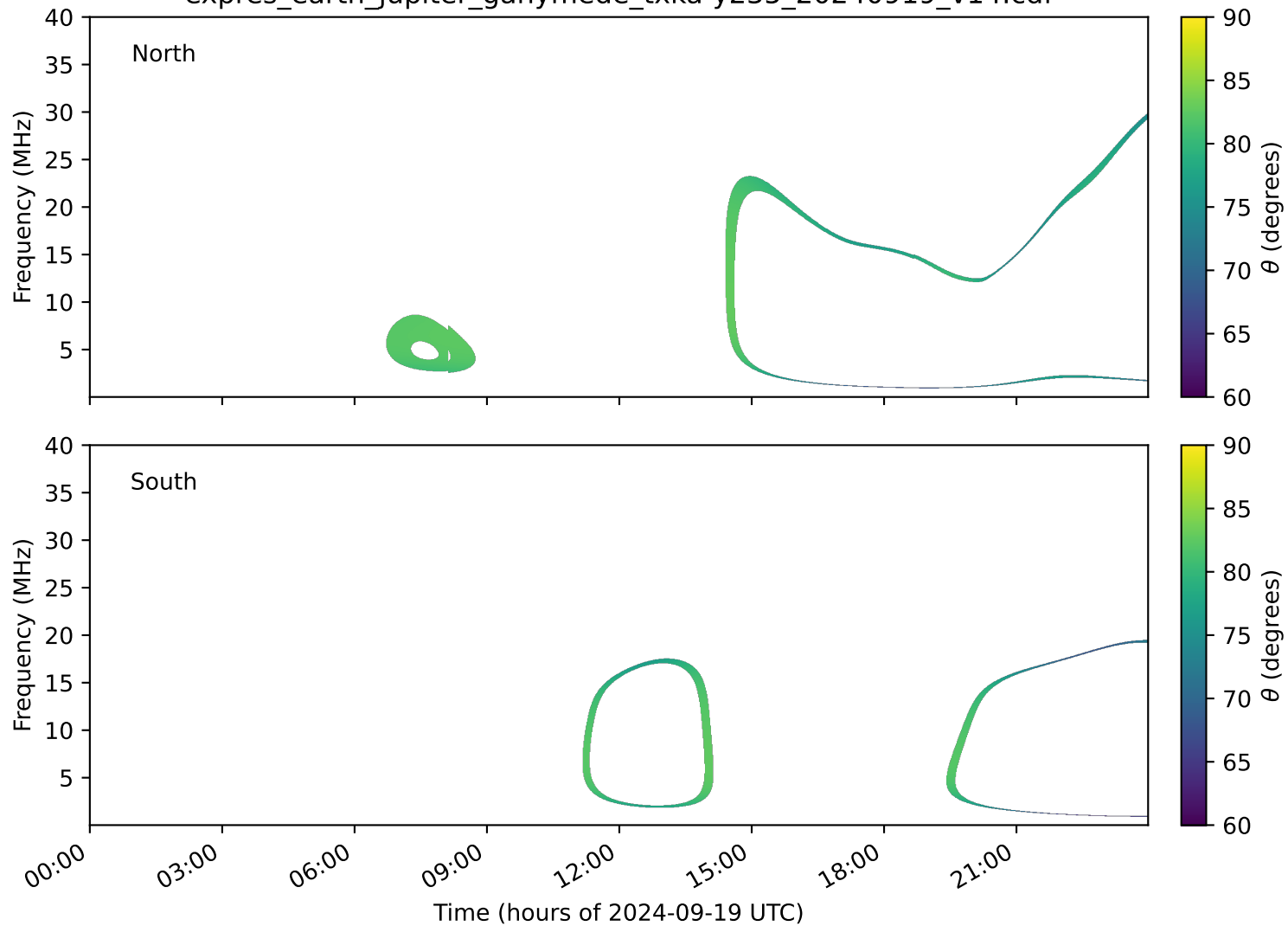
expres_earth_jupiter_ganymede_txka-y235_20240919_v14.cdf
