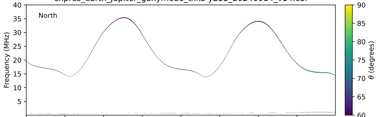
expres_earth_jupiter_ganymede_txka-y235_20240914_v14.cdf
