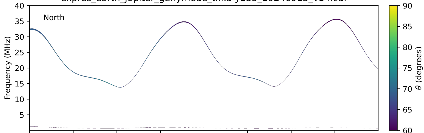
expres_earth_jupiter_ganymede_txka-y235_20240913_v14.cdf
