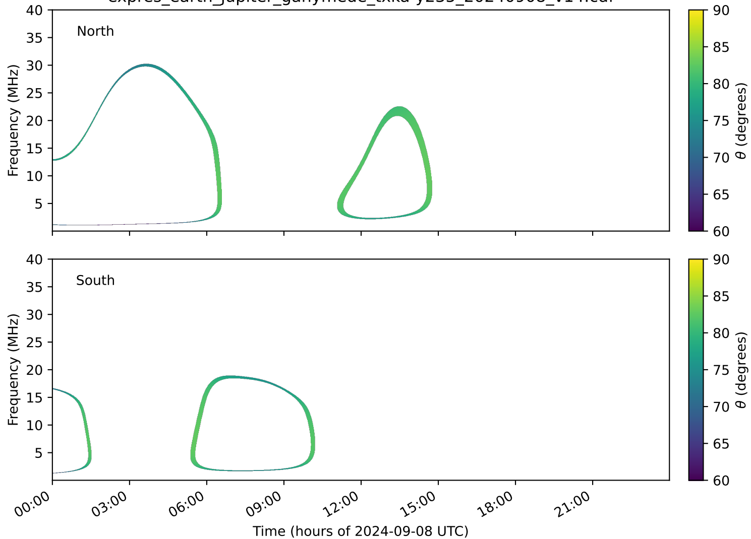
expres_earth_jupiter_ganymede_txka-y235_20240908_v14.cdf
