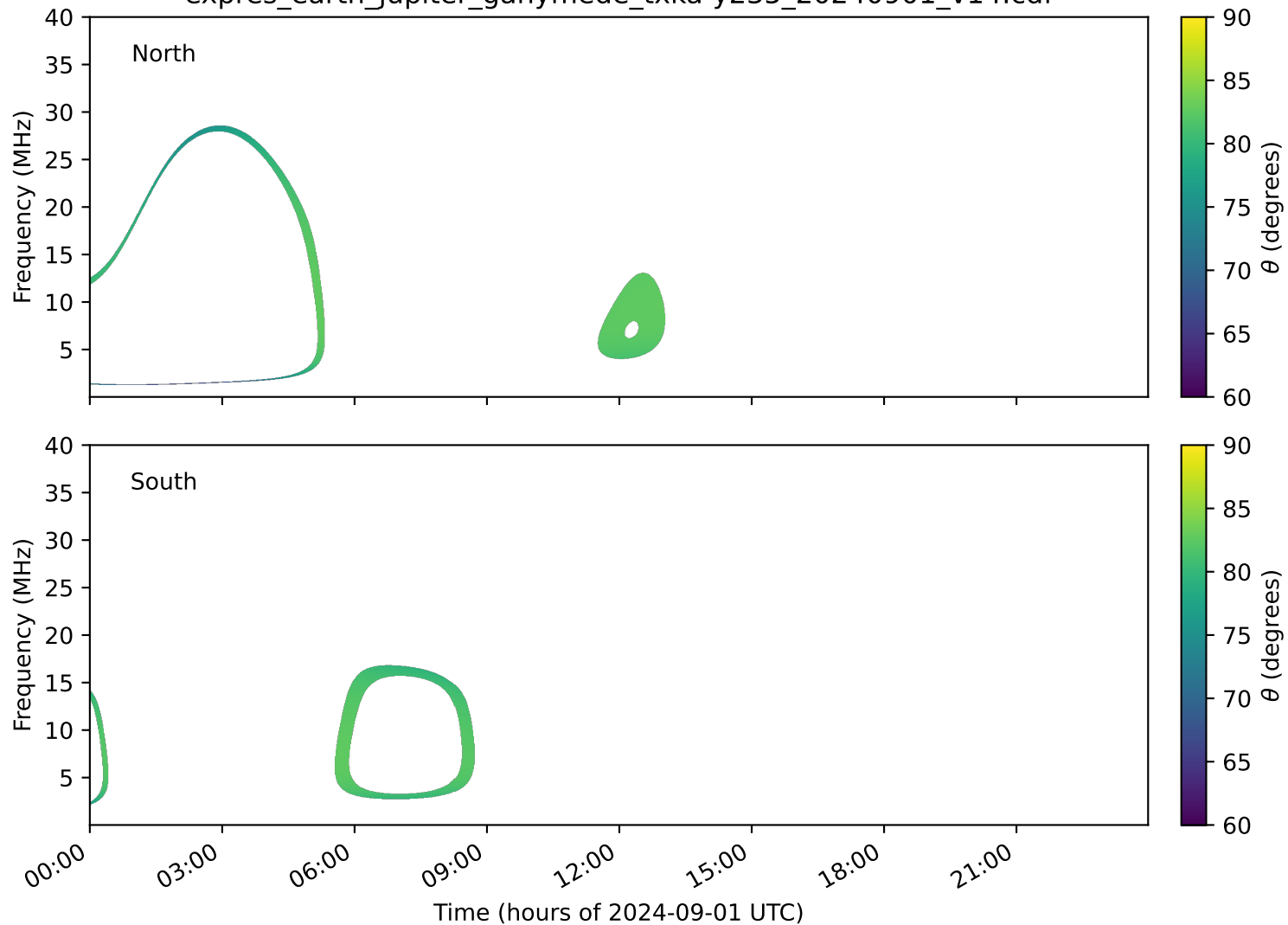
expres_earth_jupiter_ganymede_txka-y235_20240901_v14.cdf
