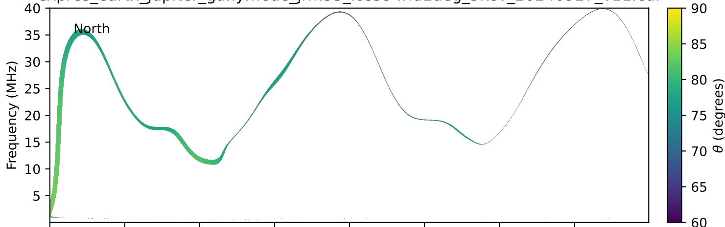
expres_earth_jupiter_ganymede_jrm33_lossc-wid1deg_3kev_20240927_v11.cdf
