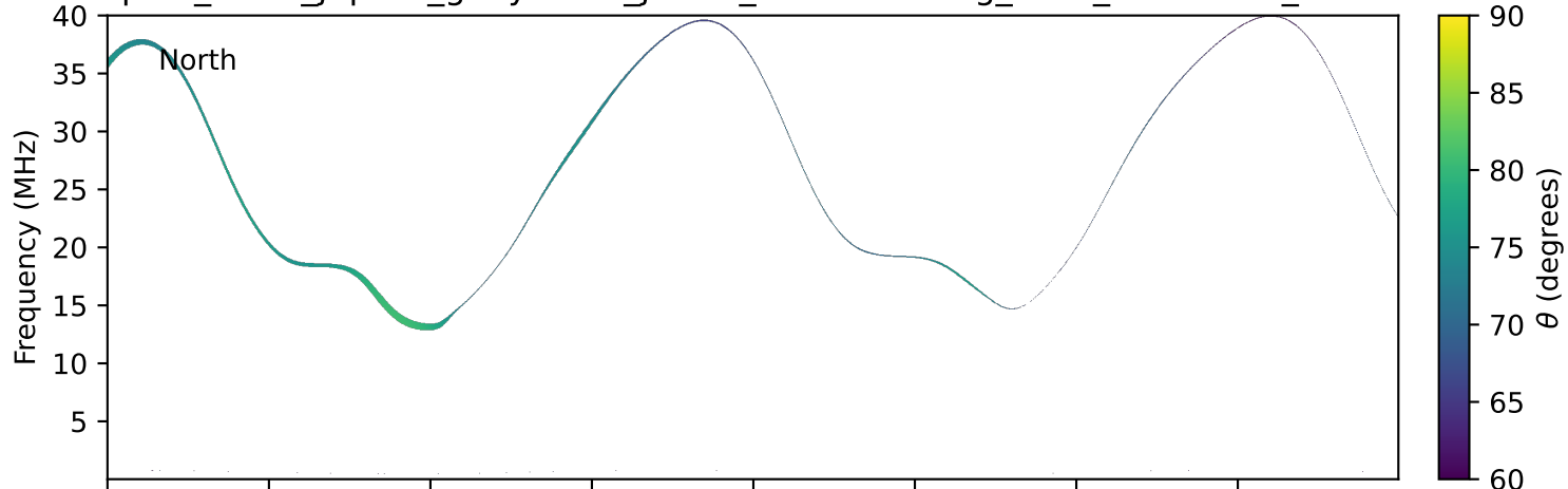
expres_earth_jupiter_ganymede_jrm33_lossc-wid1deg_3kev_20240920_v11.cdf
