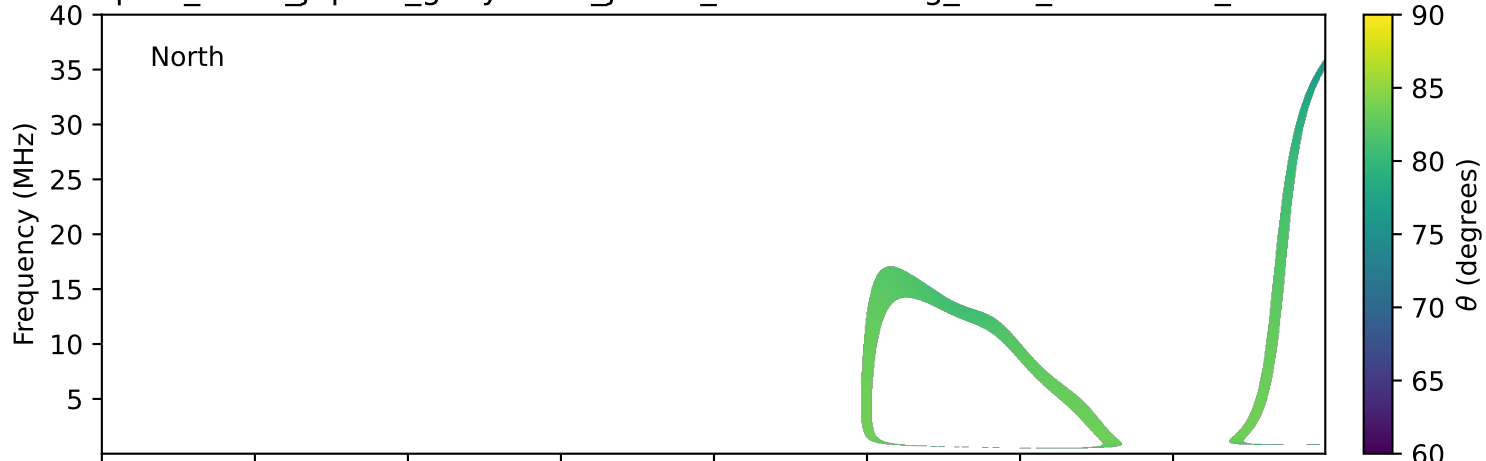
expres_earth_jupiter_ganymede_jrm33_lossc-wid1deg_3kev_20240919_v11.cdf
