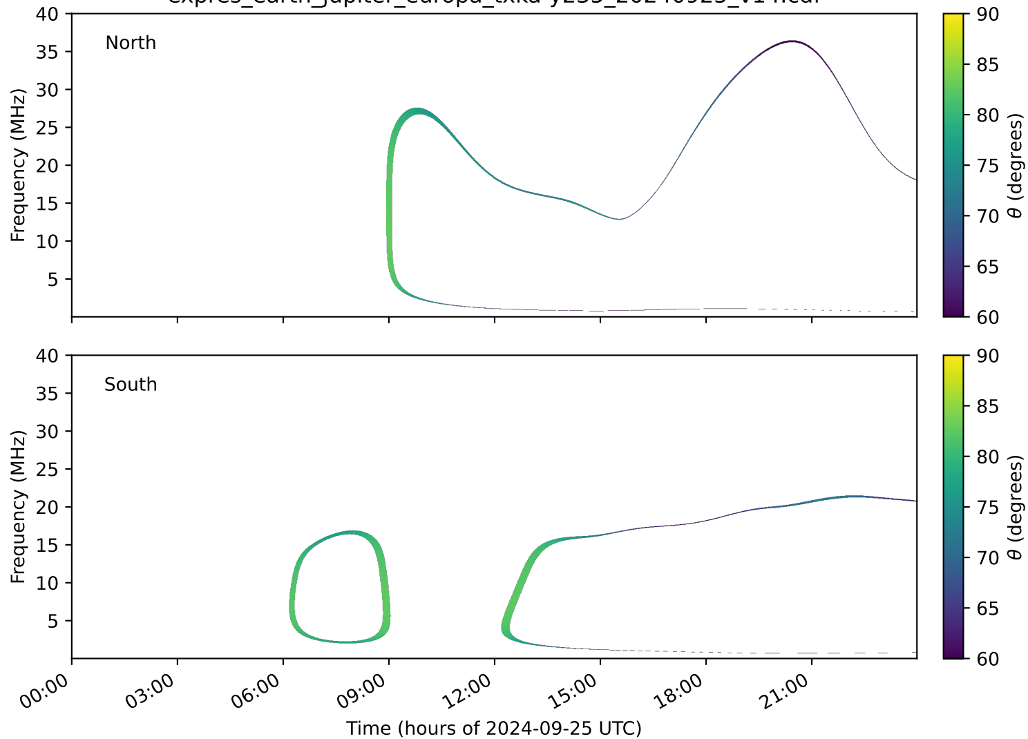
expres_earth_jupiter_europa_txka-y235_20240925_v14.cdf
