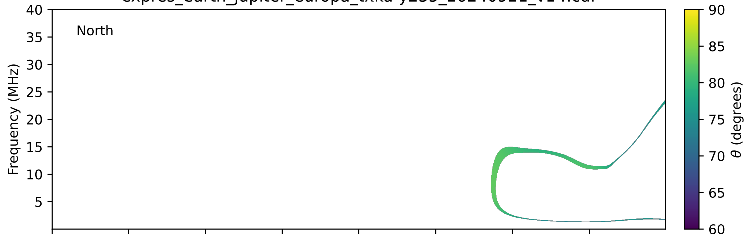
expres_earth_jupiter_europa_txka-y235_20240921_v14.cdf
