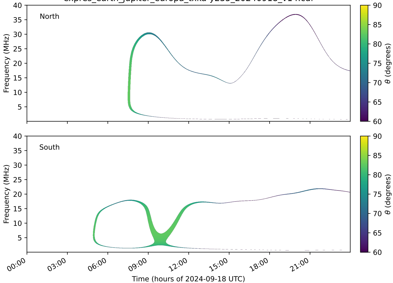
expres_earth_jupiter_europa_txka-y235_20240918_v14.cdf
