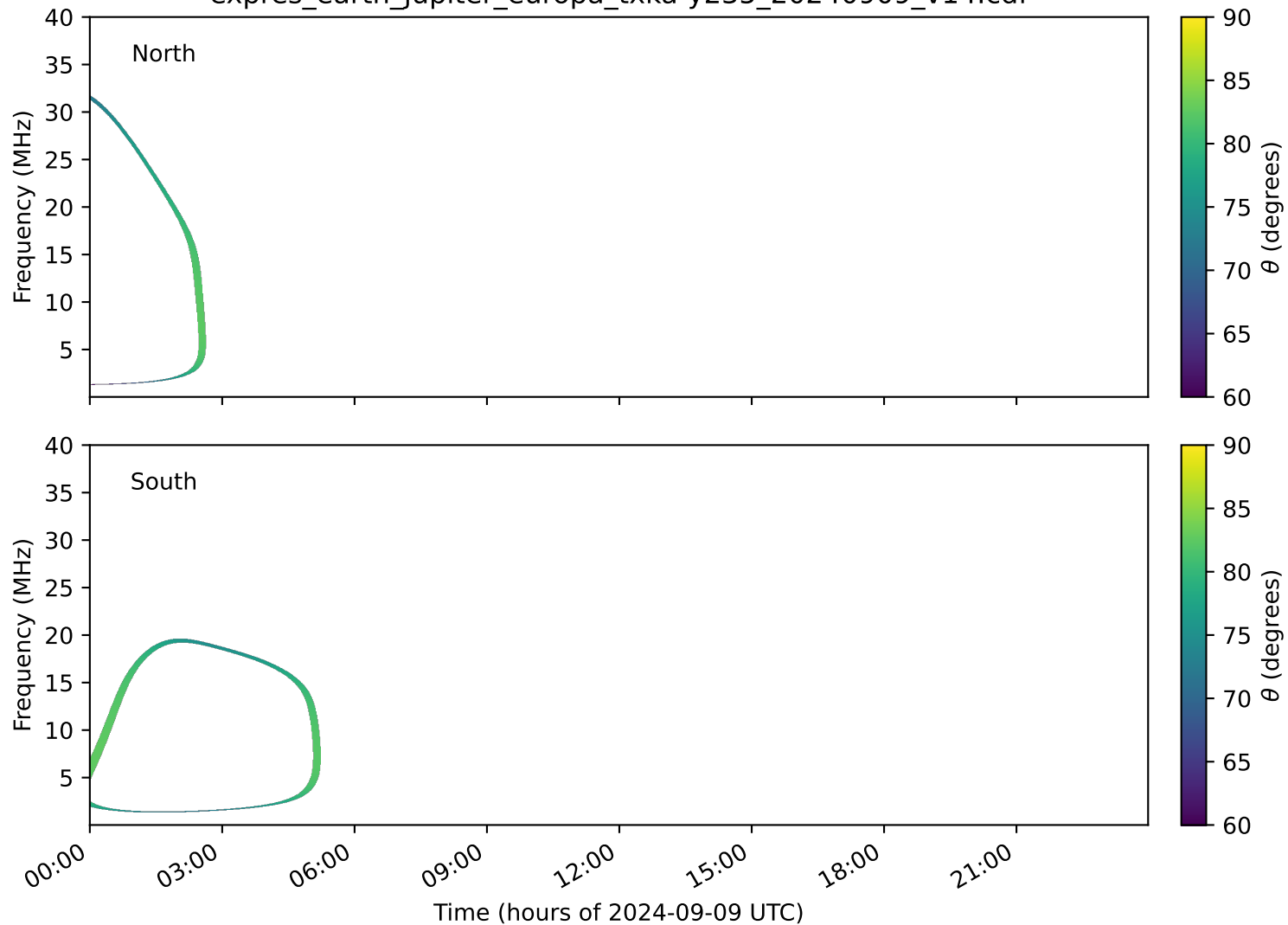
expres_earth_jupiter_europa_txka-y235_20240909_v14.cdf
