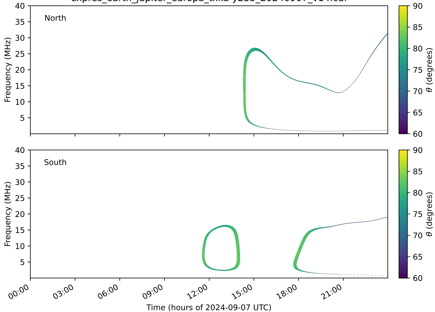
expres_earth_jupiter_europa_txka-y235_20240907_v14.cdf
