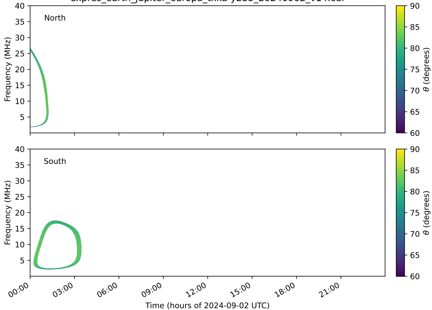
expres_earth_jupiter_europa_txka-y235_20240902_v14.cdf
