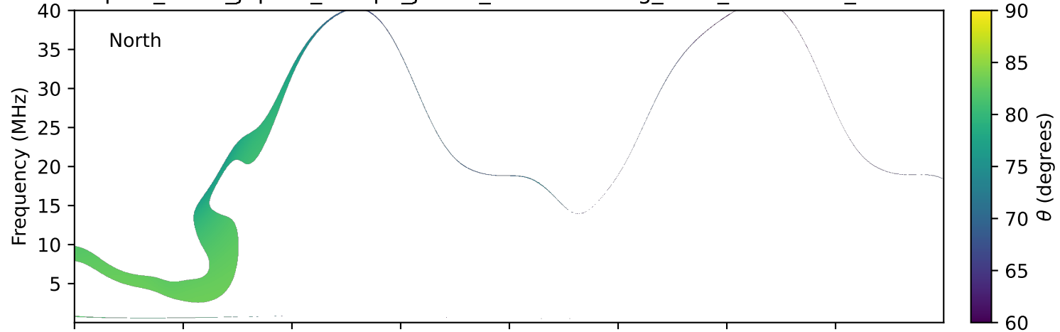
expres_earth_jupiter_europa_jrm33_lossc-wid1deg_3kev_20240904_v11.cdf
