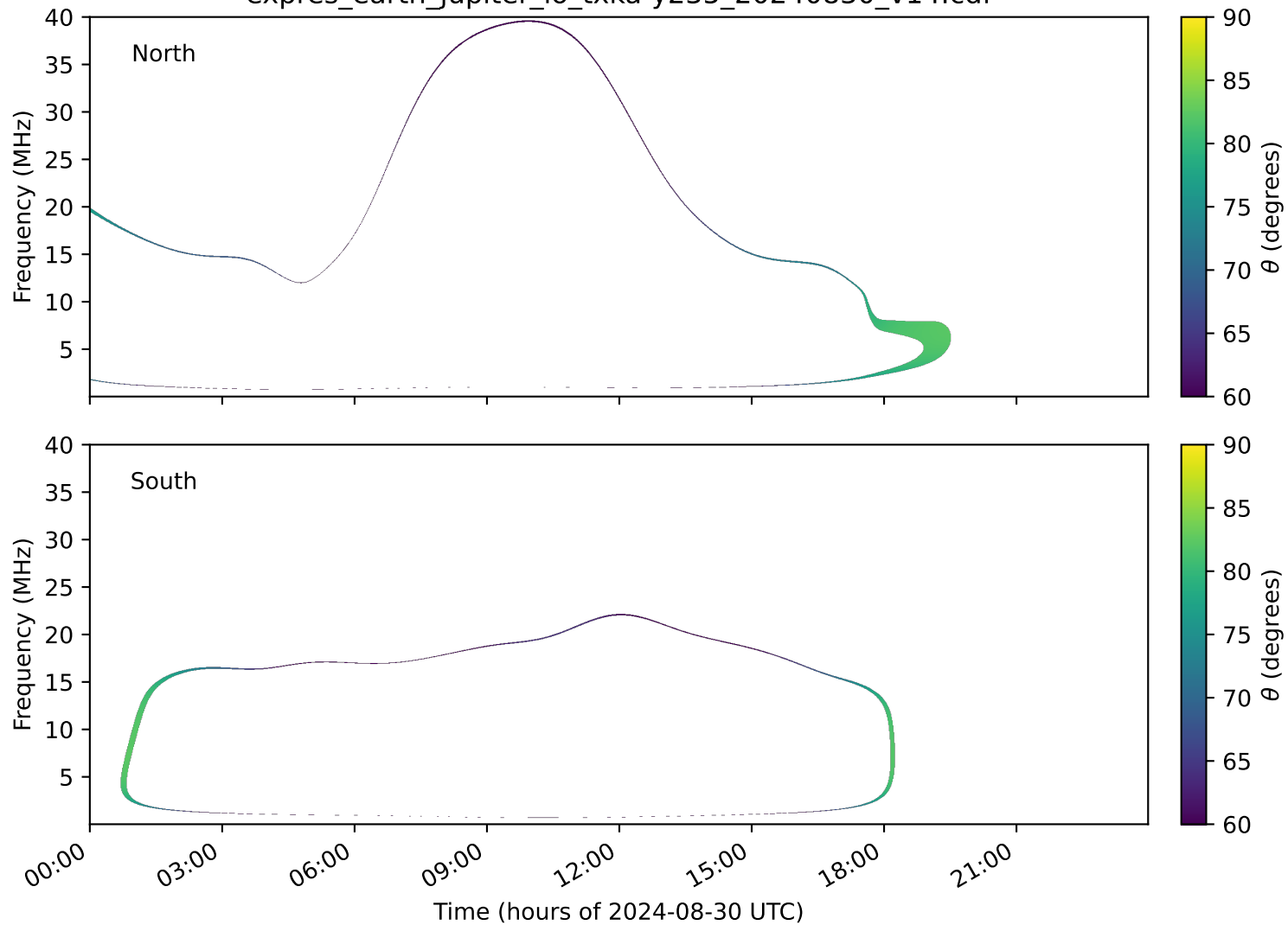
expres_earth_jupiter_io_txka-y235_20240830_v14.cdf
